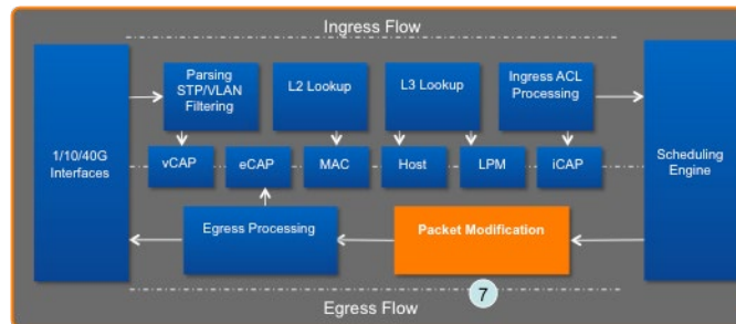
Figure 11: Packet Processor stage 7 - Packet Modification
